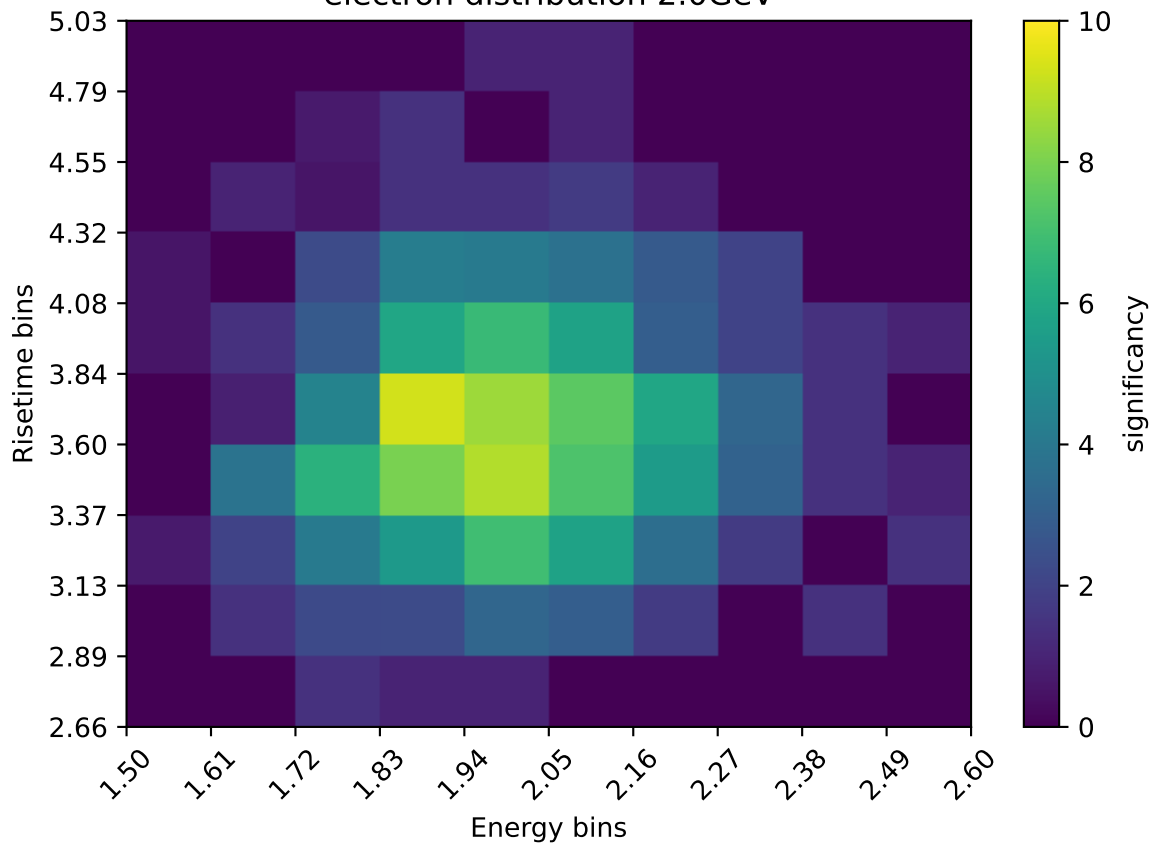
electron distribution 2.0GeV
